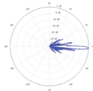
Vertical Elevation
